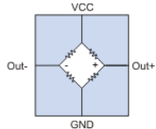
A differential bridge output
