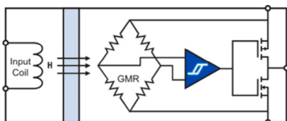
IL6xxCMTI Block Diagram (each channel).
